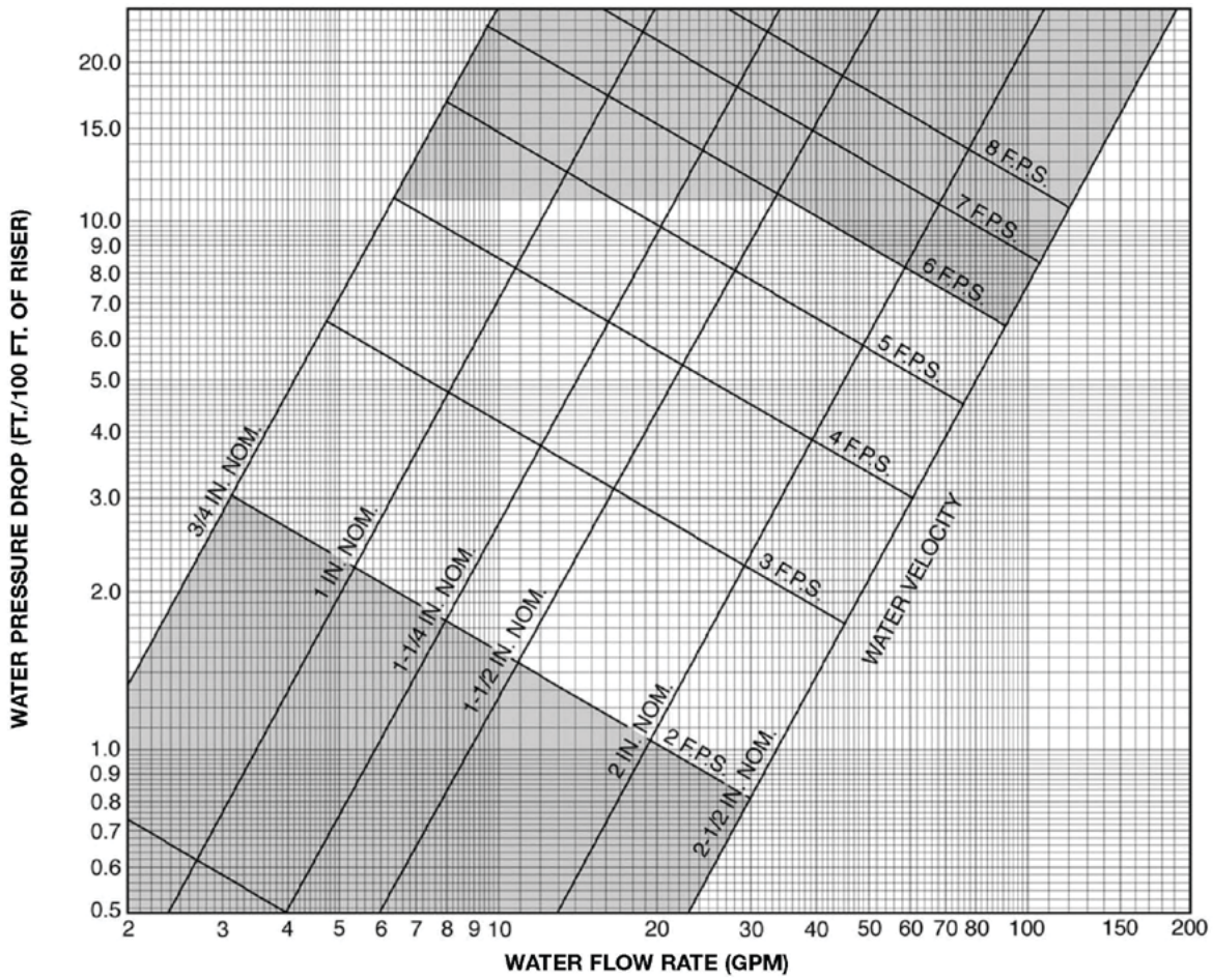
Figure 4. Type "L" Copper Riser Pressure Drop
