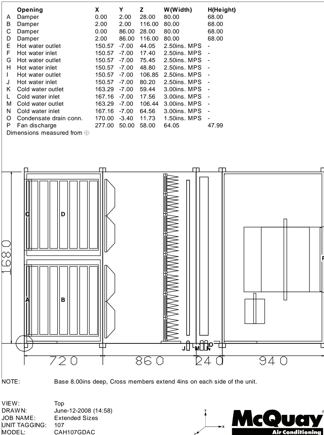
Figure 26: 107 Extended Size Drawings (Continued)
