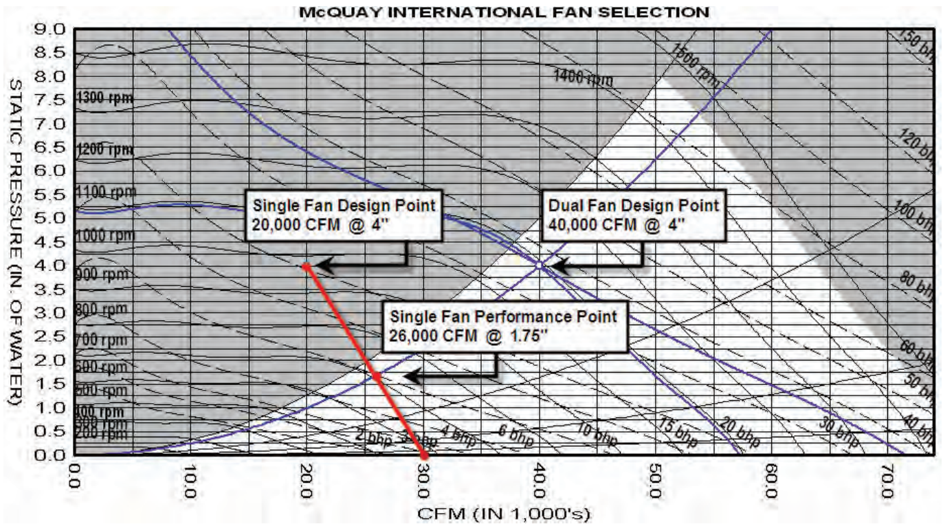
Figure 7: Dual Fan Redundancy – 65% if one fan fails
