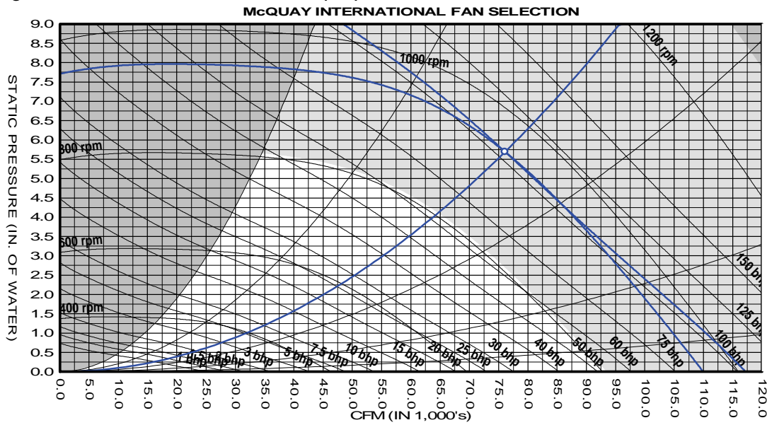
Figure 31: 160 Extended Size Fan Curve (49")
