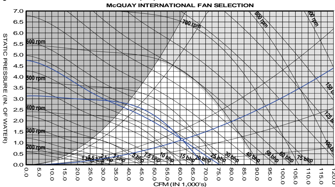
Figure 32: 160 Extended Size Fan Curve (66")
