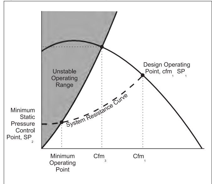
Figure 18: Variable Frequency Drive Control
