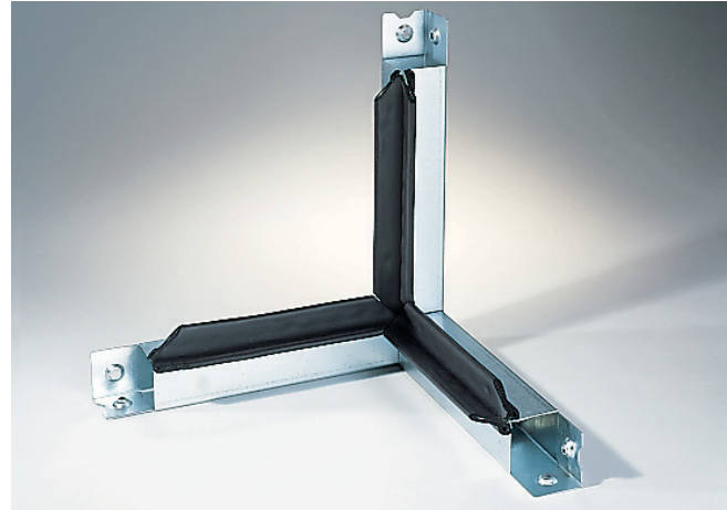
Figure 2: Patented Gasketed Frame Channel
