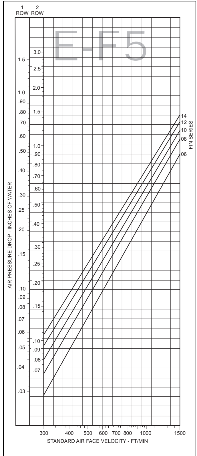
Figure 22: Coil Air Pressure Drop—E-F5 Fin Type
