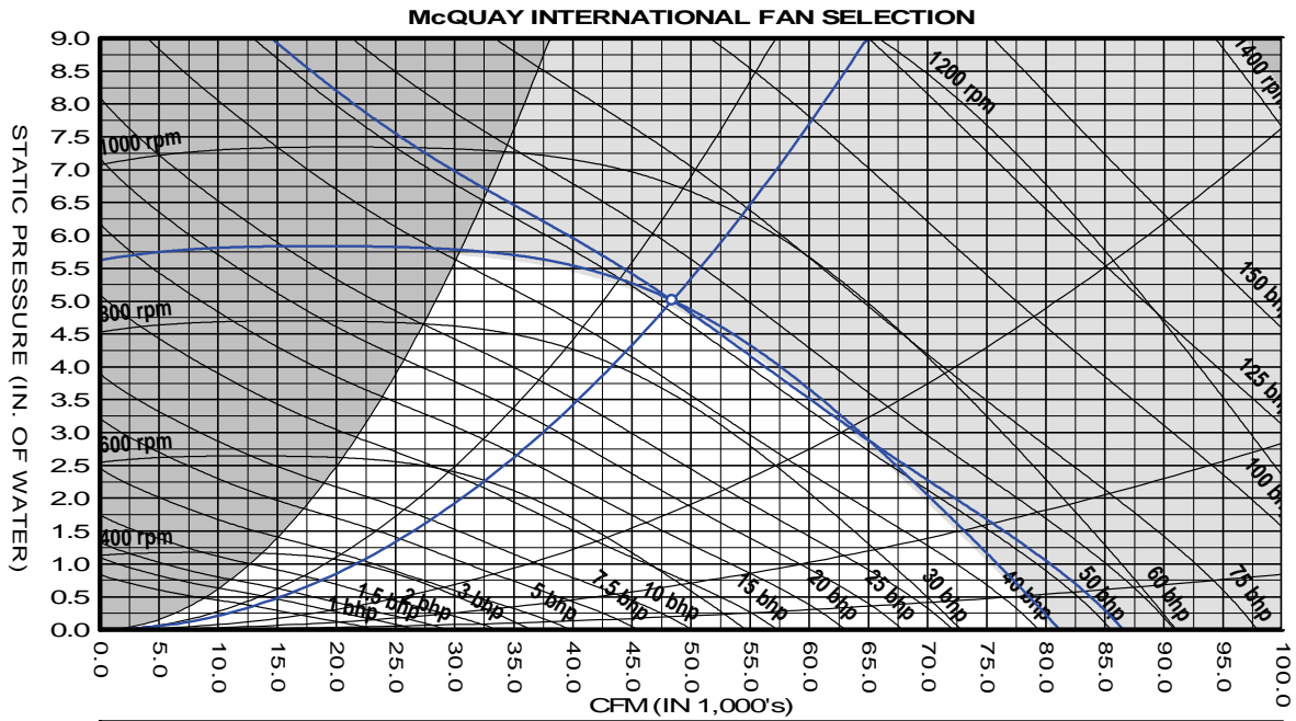
Figure 27: 107 Extended Size Fan Curve
