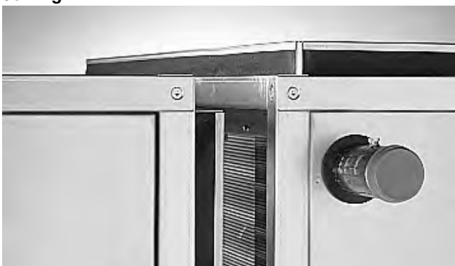
Figure 4: Patented Splice Joint for Section-to-Section Joining
