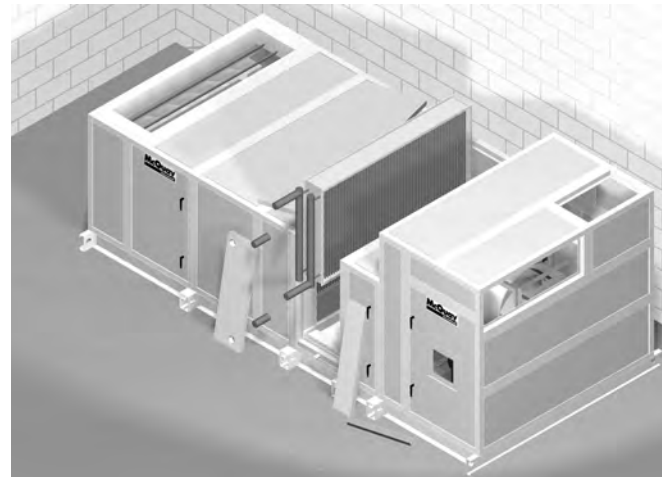
Figure 5: Panel/Channel Removal for Access
