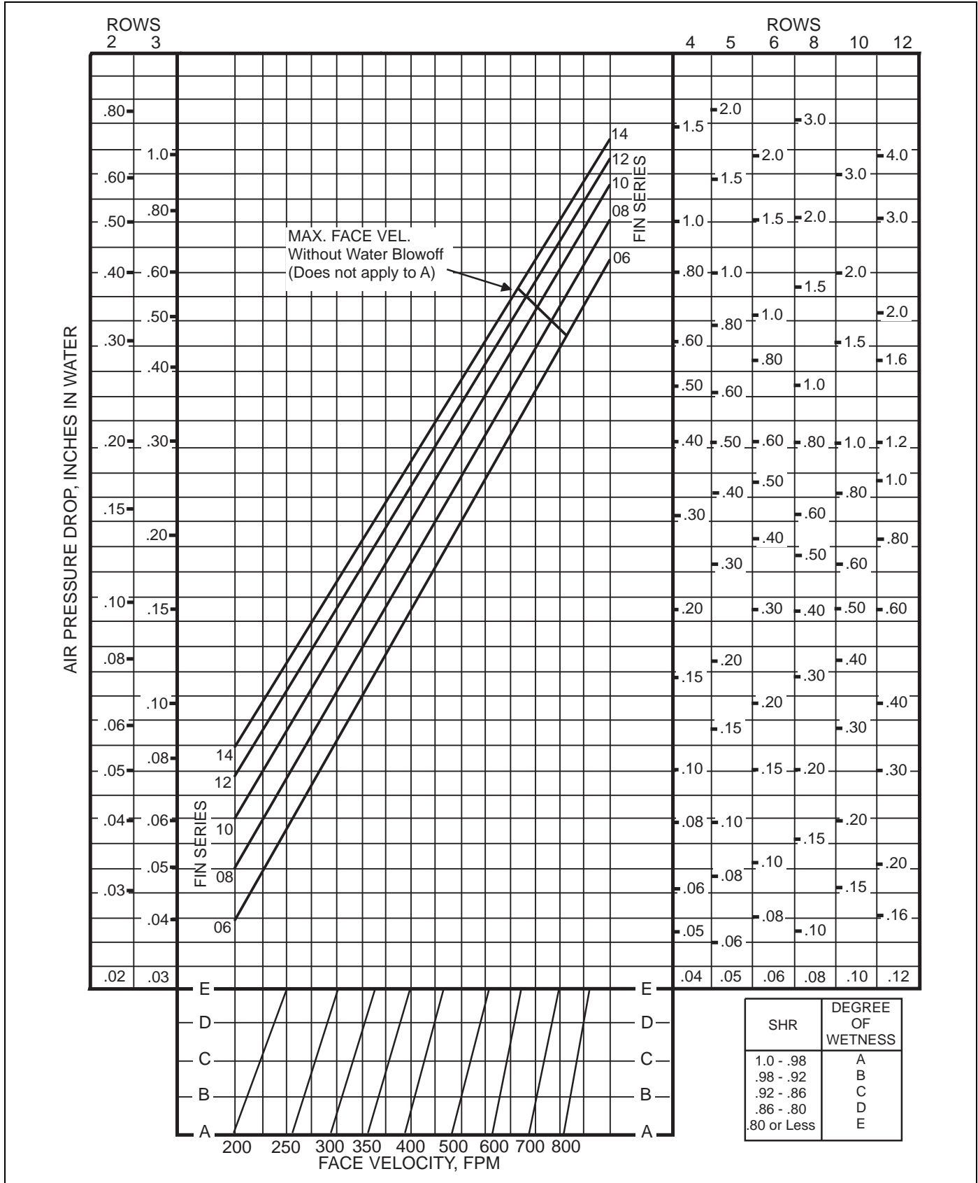
Figure 20: Coil Air Pressure Drop—E-F5 Fin Type (2 Through 12 Rows)
