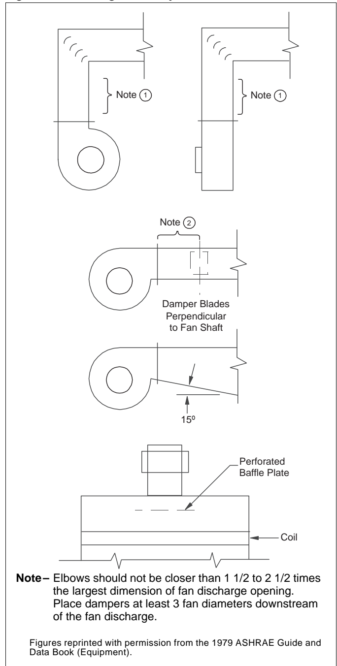
Figure 15: Discharge Duct Layout
