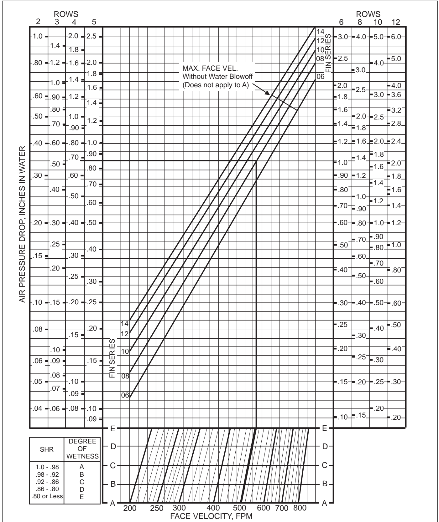
Figure 19: Coil Air Pressure Drop—HI-F5 Fin Type (2 Through 12 Rows)
