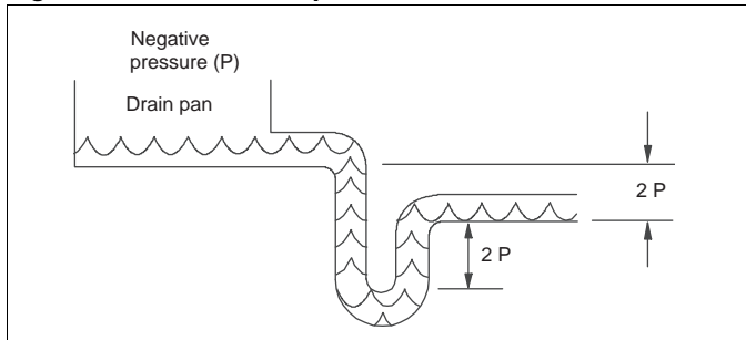
Figure 16: Drain Pan Traps
