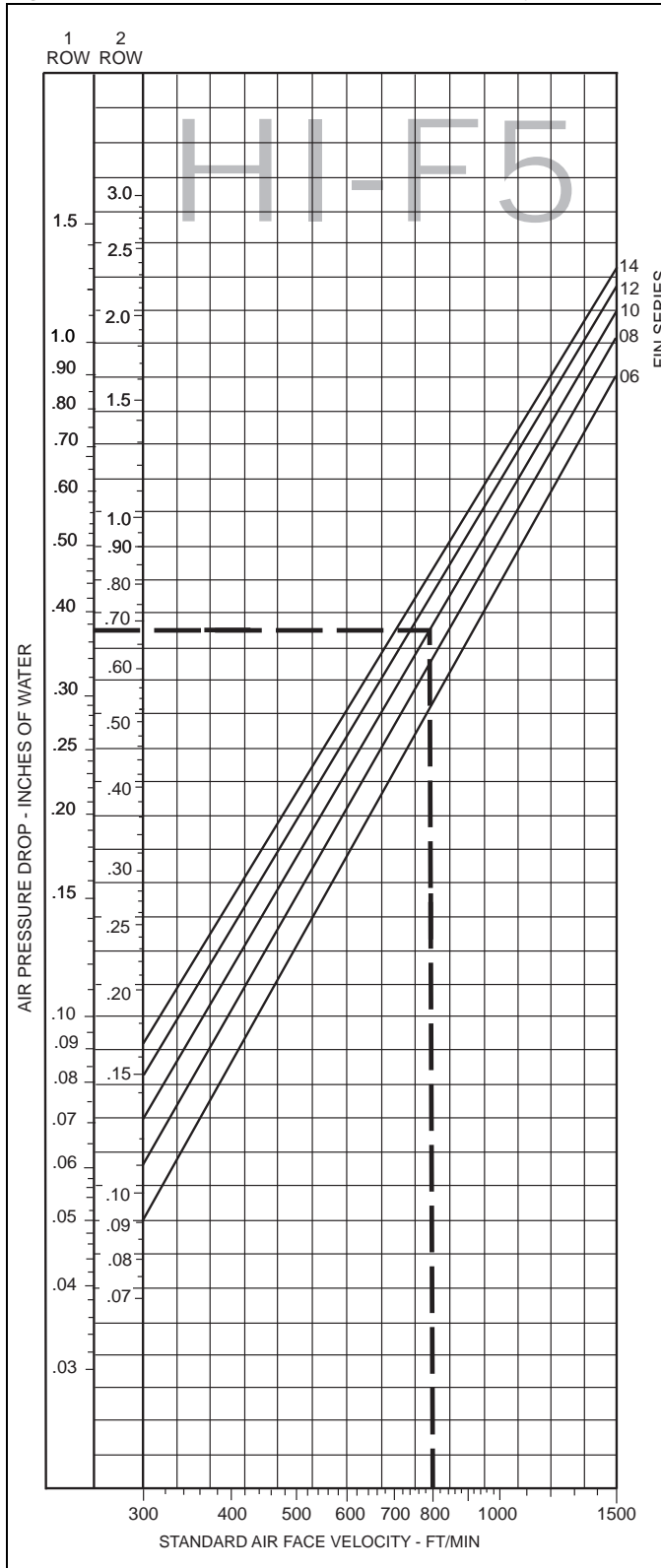
Figure 21: Coil Air Pressure Drop—HI-F5 Fin Type
